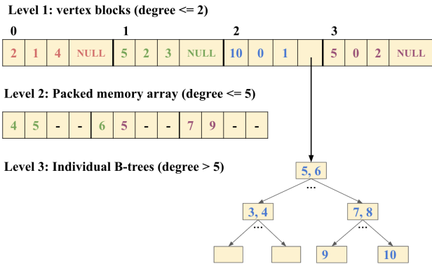
(b) An example showing how vertices of different degrees are stored in Terrace. Specifically, we show how Terrace stores vertices 0-3 from the graph in Figure 5a when S=2, L=3 . The first level is an array of vertex blocks. The second level is a shared PMA, and the last level consists of individual per-vertex B-trees.
