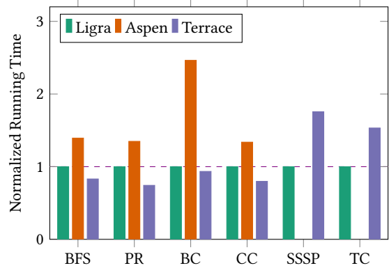
Figure 3: Average time to run kernels across all graphs in Ligra, Aspen, and Terrace normalized to Ligra. The four kernels tested for all systems were breadth-first search (BFS), PageRank (PR), single-source betweenness centrality (BC), and connected components (CC). Aspen does not have publicly available implementations of single-source shortest paths (SSSP) or triangle counting (TC), so we omit it from SSSP and TC.
